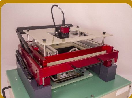
PNEUMATIC FIXTURE PCB TESTING
